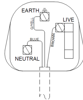
5 AMP 230V PLUG BS1363
